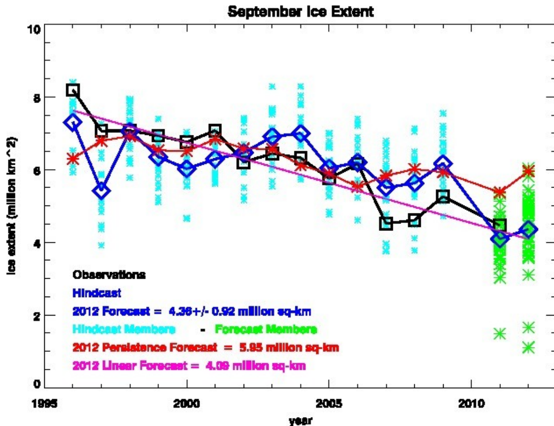
Figure 1: September sea ice extents (million km 2 ) from the GloSea4 seasonal forecasting system, for hindcasts initialised on 9 th and 17 th March, and 1 st April, and forecasts initialised between March 12 th and April 1 st . All values (except the observations) have been bias-corrected. The persistence forecast values are generated by applying the mean observed anomaly in March ice extent each year to the September climatology.
