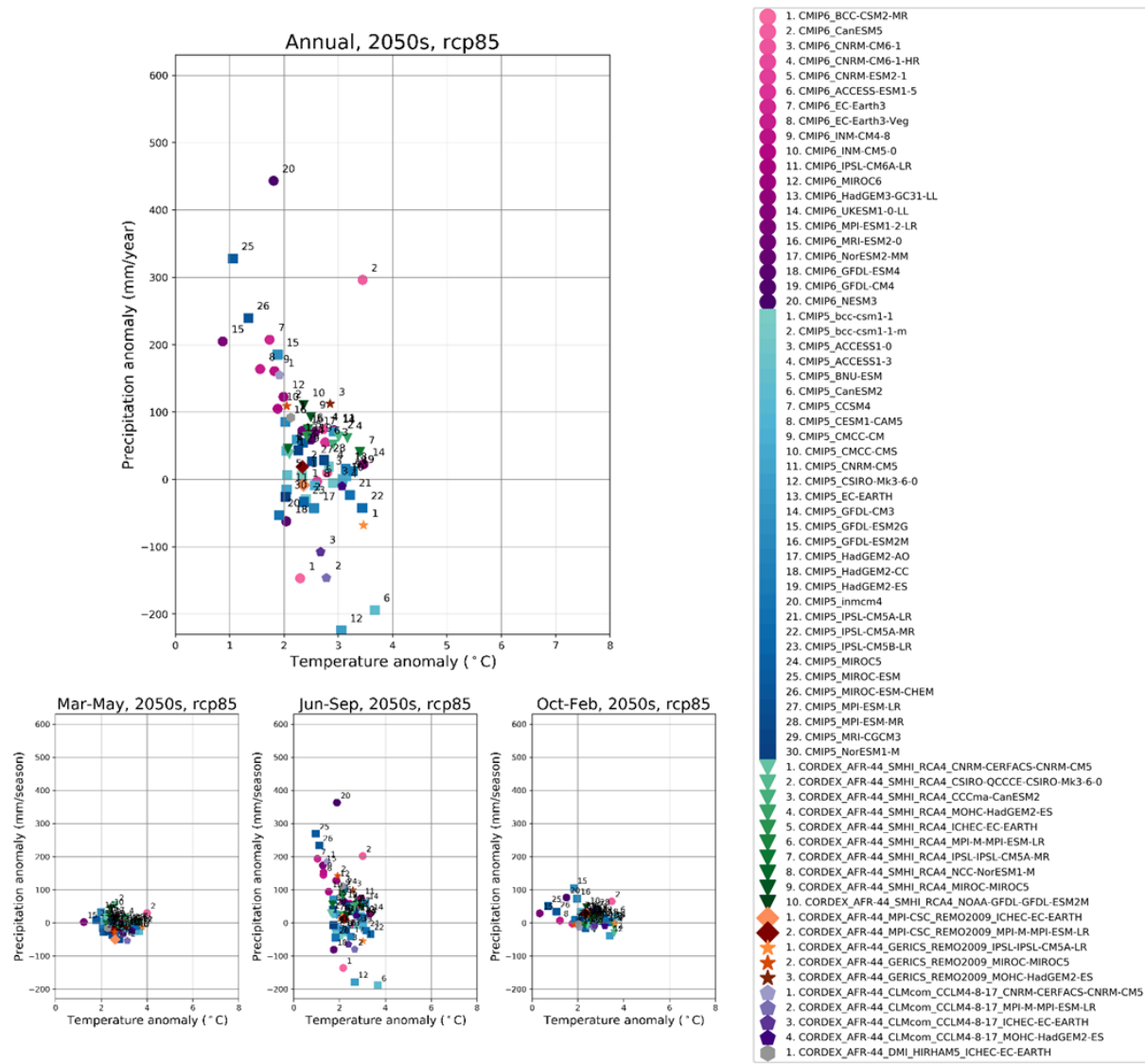
Figure B12: Projected change in average annual (top panel) and seasonal (bottom panels) precipitation and temperature in Zone 1. Each dot shows the difference between the average projected values in the 2050s and the average values in the current climate, for each climate model. Individual models are identified by the icon and number in the legend.
