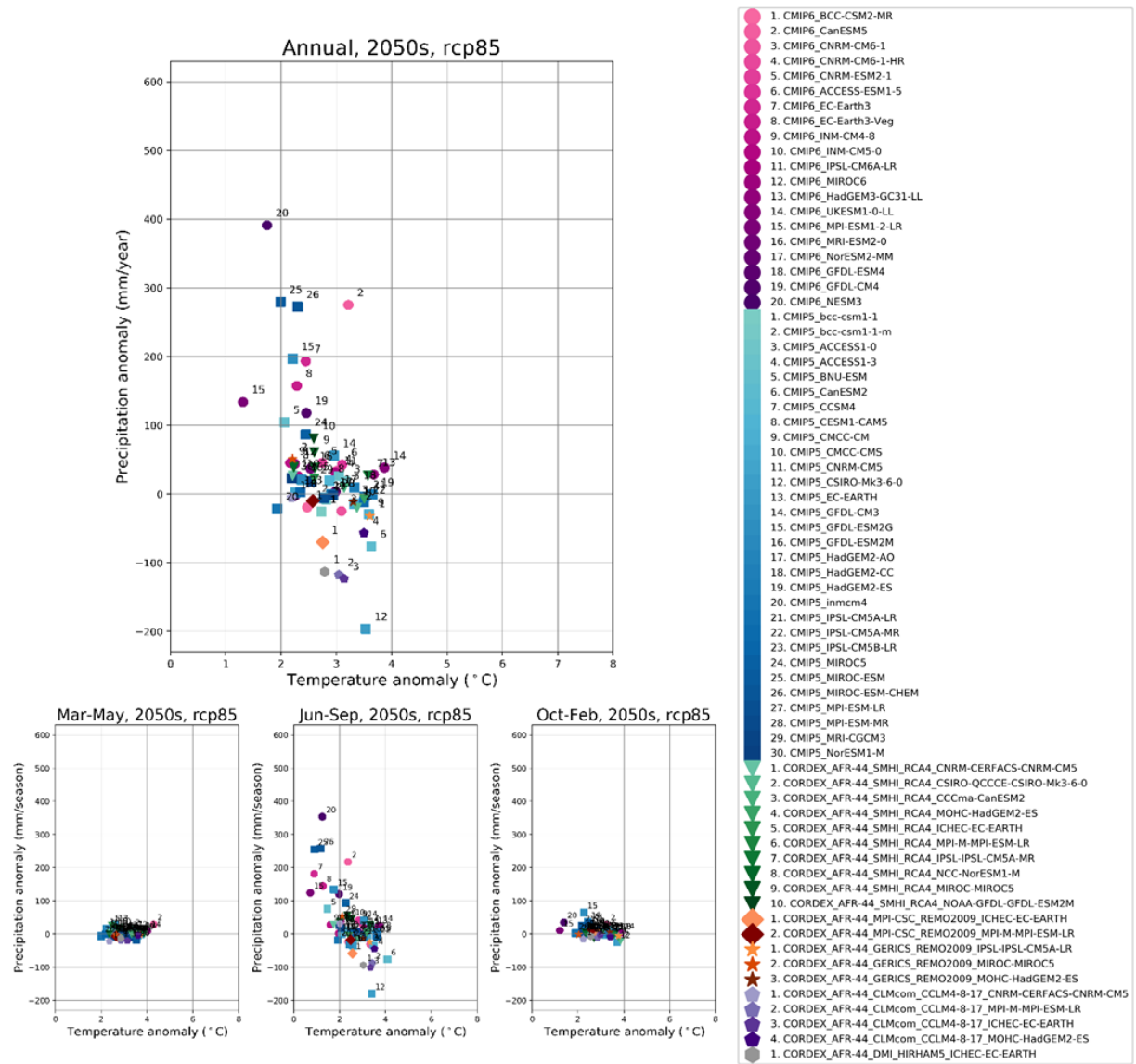
Figure B8: Projected change in average annual (top panel) and seasonal (bottom panels) precipitation and temperature in Zone 1. Each dot shows the difference between the average projected values in the 2050s and the average values in the current climate, for each climate model. Individual models are identified by the icon and number in the legend.
