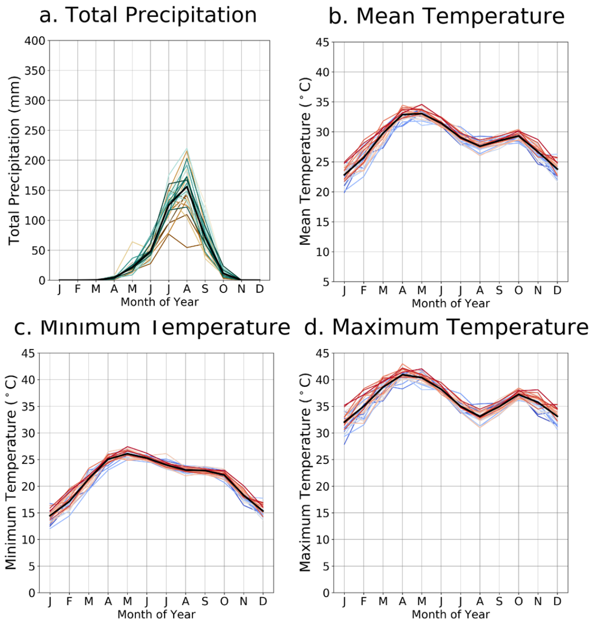
Figure B9: Observations of total monthly precipitation (a) and average daily mean (b), minimum (c) and maximum (d) temperature over the baseline period (1981-2010) for Zone 1. Each line is one individual year. Colours show the ordering of years from brown-blue (total precipitation) and blue-red (mean temperature) – this highlights the presence, or lack of, a trend over the baseline period. The bold black line indicates the average of the 30-year period. Observational dataset: CHIRPS and WFDEI for precipitation and temperature respectively.
