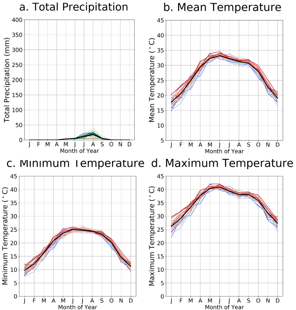
Figure B5: Observations of total monthly precipitation (a) and average daily mean (b), minimum (c) and maximum (d) temperature over the baseline period (1981-2010) for Zone 1. Each line is one individual year. Colours show the ordering of years from brown-blue (total precipitation) and blue-red (mean temperature) – this highlights the presence, or lack of, a trend over the baseline period. The bold black line indicates the average of the 30-year period. Observational dataset: CHIRPS and WFDEI for precipitation and temperature respectively.
