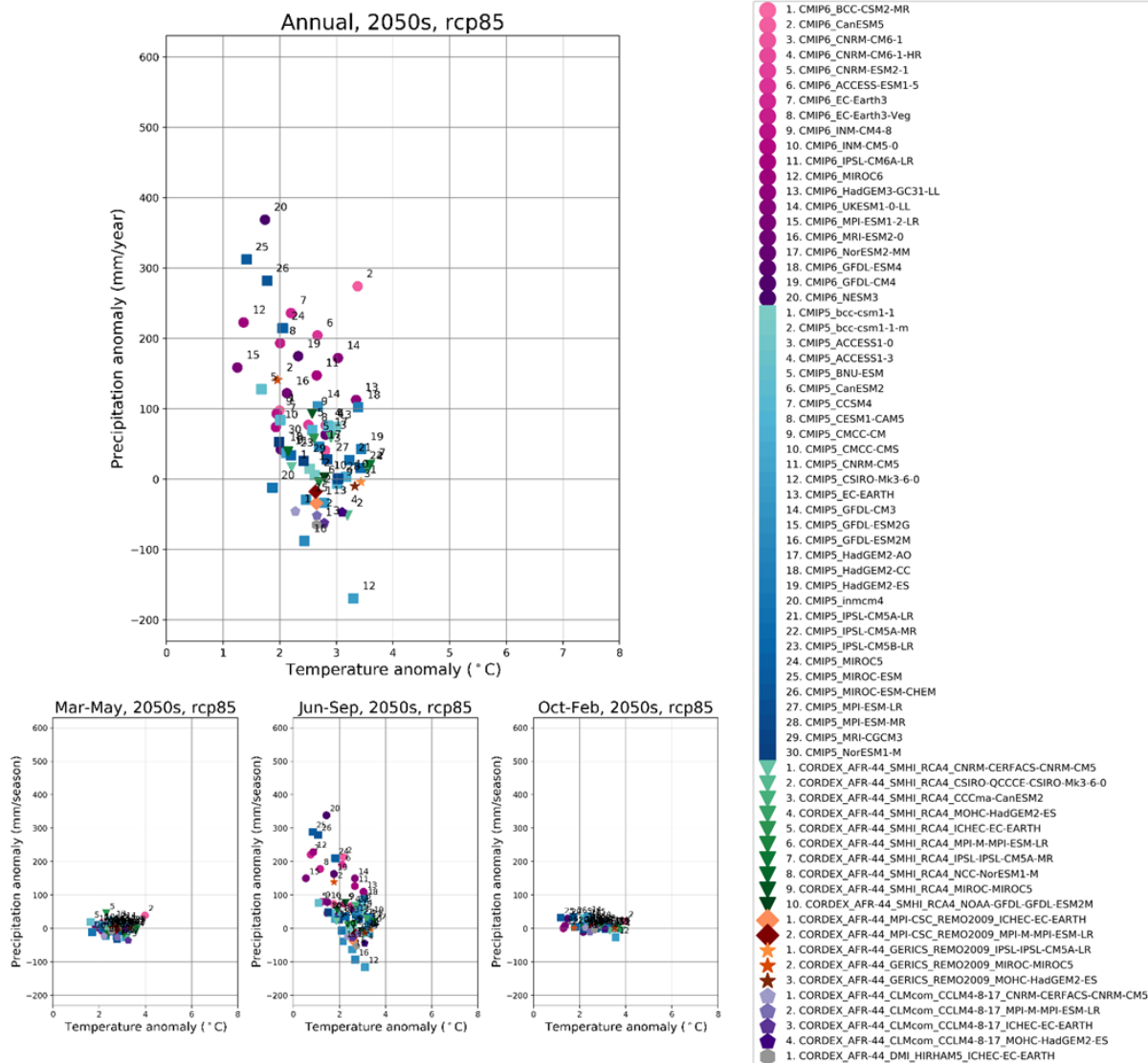
Figure B10: Projected change in average annual (top panel) and seasonal (bottom panels) precipitation and temperature in Zone 1. Each dot shows the difference between the average projected values in the 2050s and the average values in the current climate, for each climate model. Individual models are identified by the icon and number in the legend.
