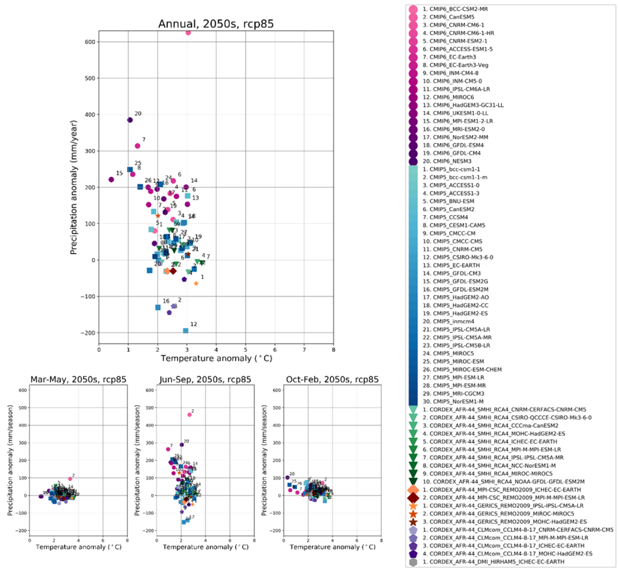
Figure B14: Projected change in average annual (top panel) and seasonal (bottom panels) precipitation and temperature in Zone 1. Each dot shows the difference between the average projected values in the 2050s and the average values in the current climate, for each climate model. Individual models are identified by the icon and number in the legend.
