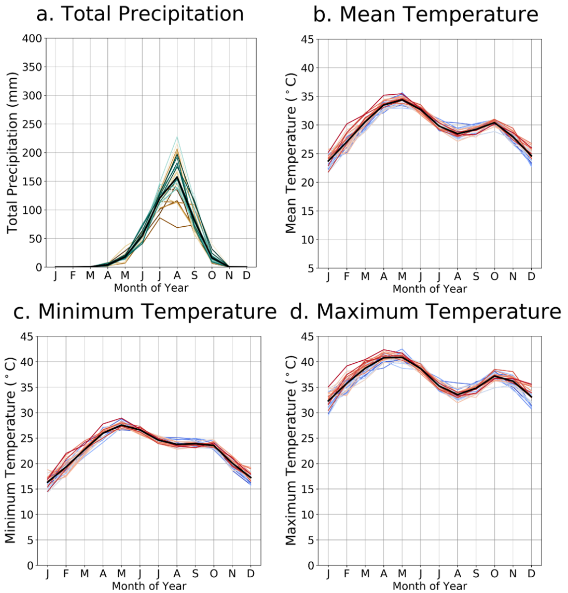
Figure B7: Observations of total monthly precipitation (a) and average daily mean (b), minimum (c) and maximum (d) temperature over the baseline period (1981-2010) for Zone 1. Each line is one individual year. Colours show the ordering of years from brown-blue (total precipitation) and blue-red (mean temperature) – this highlights the presence, or lack of, a trend over the baseline period. The bold black line indicates the average of the 30-year period. Observational dataset: CHIRPS and WFDEI for precipitation and temperature respectively.
