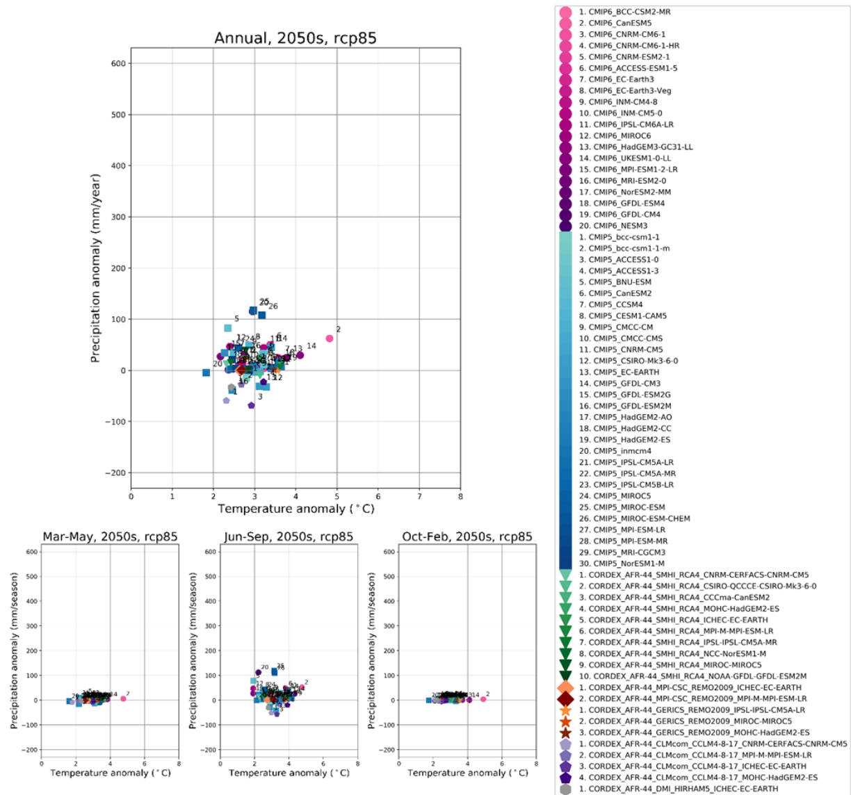
Figure B6: Projected change in average annual (top panel) and seasonal (bottom panels) precipitation and temperature in Zone 1. Each dot shows the difference between the average projected values in the 2050s and the average values in the current climate, for each climate model. Individual models are identified by the icon and number in the legend.
