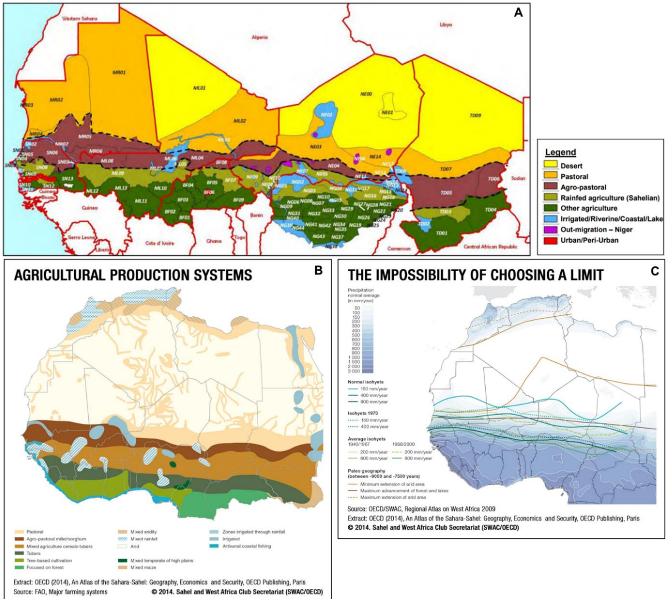
Figure B2: Maps used to create spatial analysis zones for Sahel region in addition to climate classification. Map A shows FEWS NET livelihoods zones overlaid with modes of agriculture including those based around major river systems (Holt & Lawrence, 2013). Map B shows simplified map of major agricultural production systems (OECD, 2014). Map C shows multiple isohyet lines for different historical periods, indicating the oversimplification of individual isohyet lines (OECD/SWAC; 2009).
