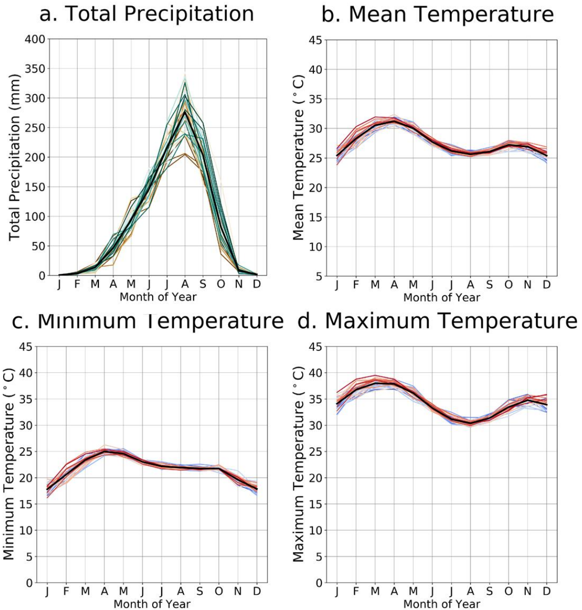
Figure B11: Observations of total monthly precipitation (a) and average daily mean (b), minimum (c) and maximum (d) temperature over the baseline period (1981-2010) for Zone 1. Each line is one individual year. Colours show the ordering of years from brown-blue (total precipitation) and blue-red (mean temperature) – this highlights the presence, or lack of, a trend over the baseline period. The bold black line indicates the average of the 30-year period. Observational dataset: CHIRPS and WFDEI for precipitation and temperature respectively.
