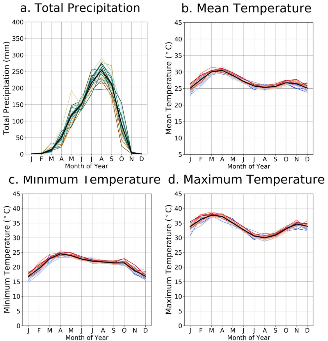
Figure B13: Observations of total monthly precipitation (a) and average daily mean (b), minimum (c) and maximum (d) temperature over the baseline period (1981-2010) for Zone 1. Each line is one individual year. Colours show the ordering of years from brown-blue (total precipitation) and blue-red (mean temperature) – this highlights the presence, or lack of, a trend over the baseline period. The bold black line indicates the average of the 30-year period. Observational dataset: CHIRPS and WFDEI for precipitation and temperature respectively.
