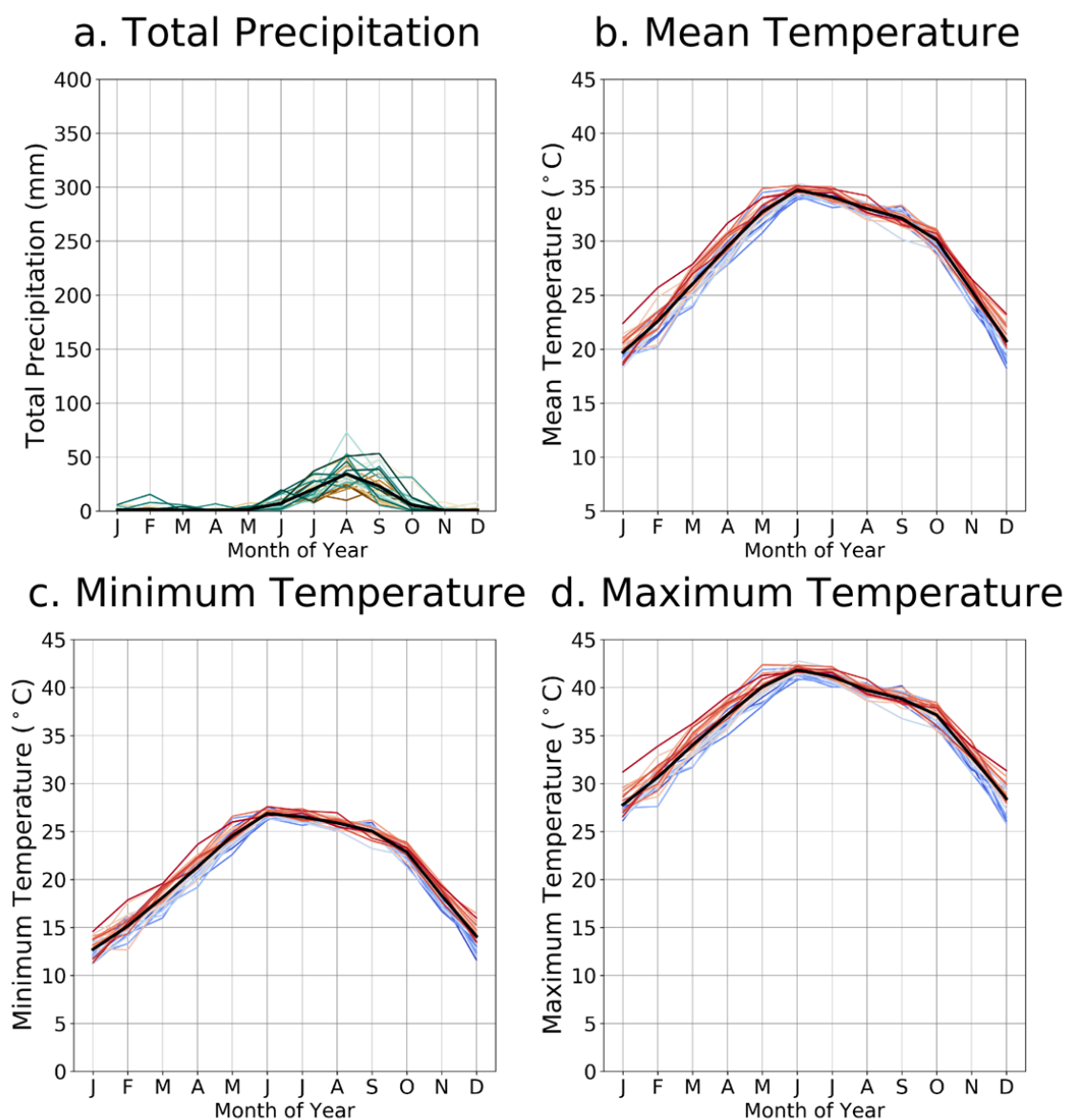
Figure B3: Observations of total monthly precipitation (a) and average daily mean (b), minimum (c) and maximum (d) temperature over the baseline period (1981-2010) for Zone 1. Each line is one individual year. Colours show the ordering of years from brown-blue (total precipitation) and blue-red (mean temperature) – this highlights the presence, or lack of, a trend over the baseline period. The bold black line indicates the average of the 30-year period. Observational dataset: CHIRPS and WFDEI for precipitation and temperature respectively.
