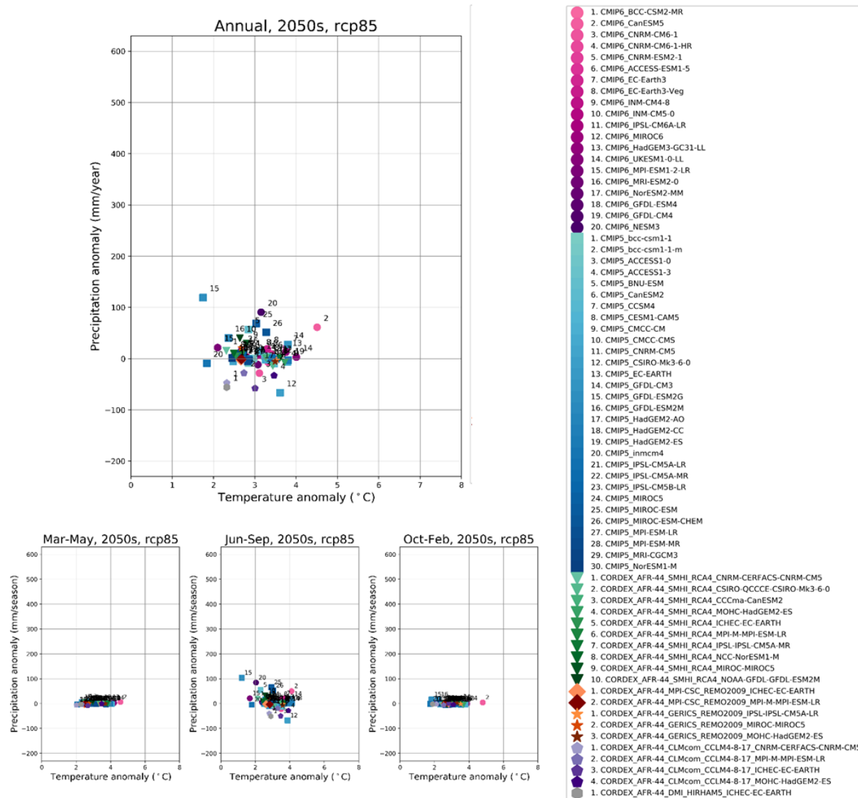
Figure B4: Projected change in average annual (top panel) and seasonal (bottom panels) precipitation and temperature in Zone 1. Each dot shows the difference between the average projected values in the 2050s and the average values in the current climate, for each climate model. Individual models are identified by the icon and number in the legend.
